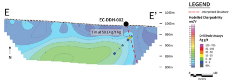
Figure 6: Cross Section looking north on IP chargeability PDP geophysics
